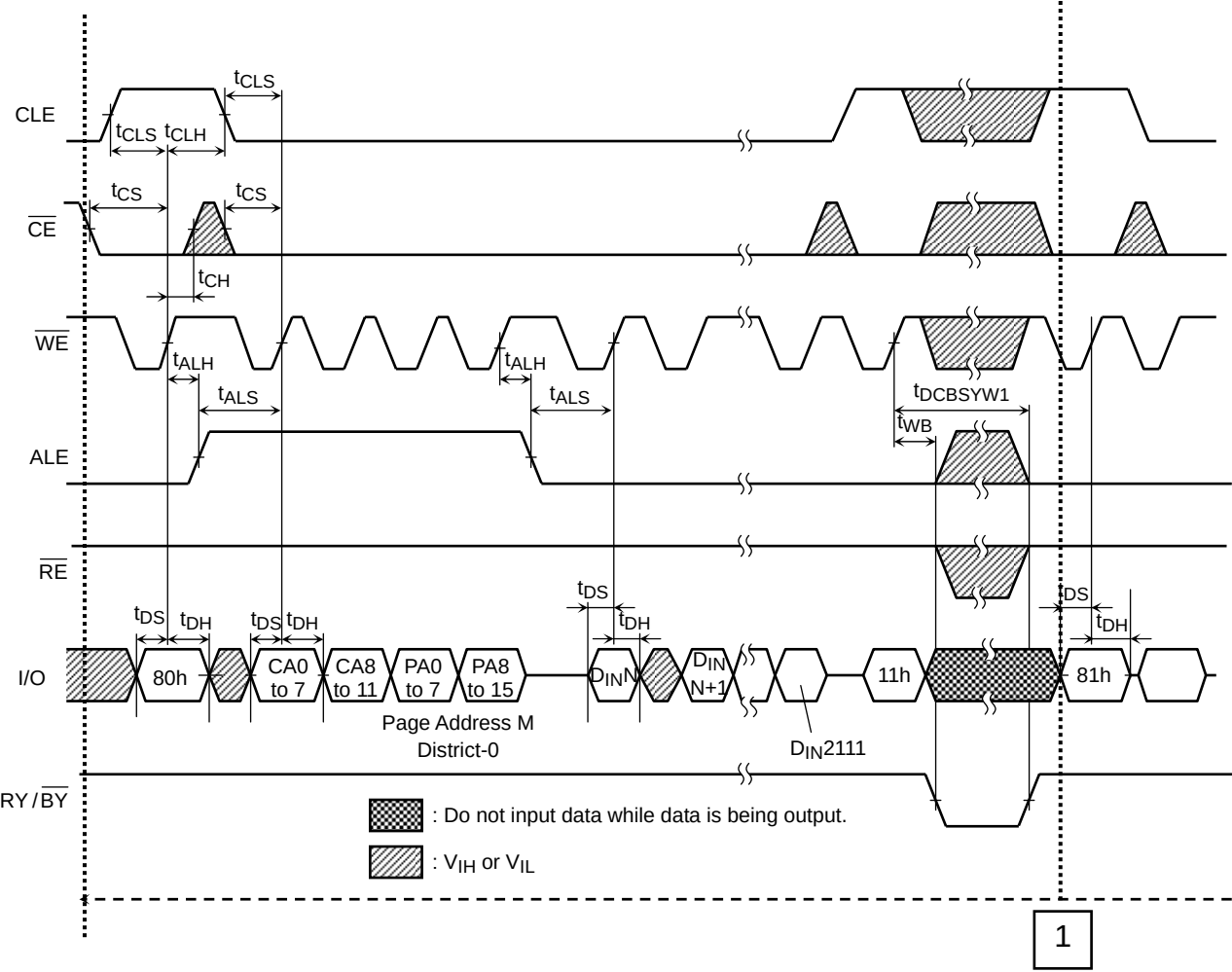
Multi-Page Program Operation with Data Cache Timing Diagram (1/4)
