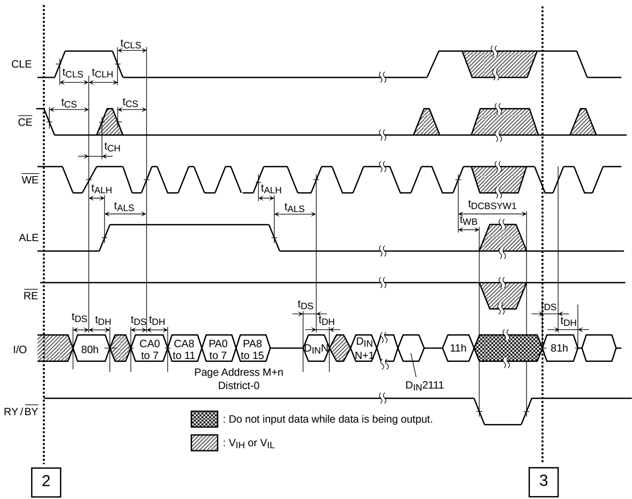
Multi-Page Program Operation with Data Cache Timing Diagram (3/4)
